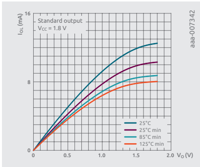
I_{OI} at 1.8V
