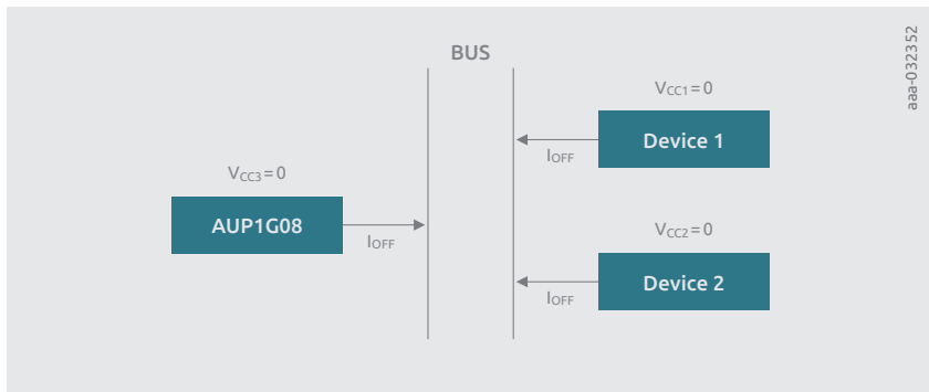
Figure 5.15 | Bus system with Logic devices featuring I OFF
