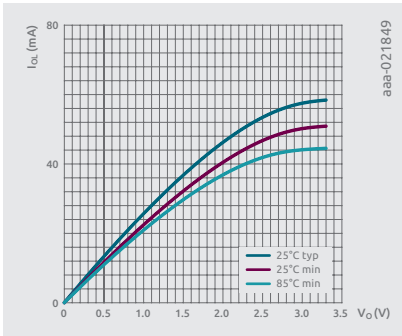
I_{OL} at 3.5V
