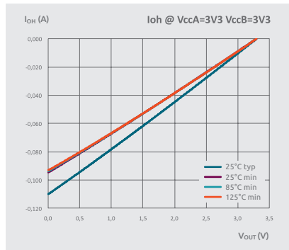
AVC output at 3V3
