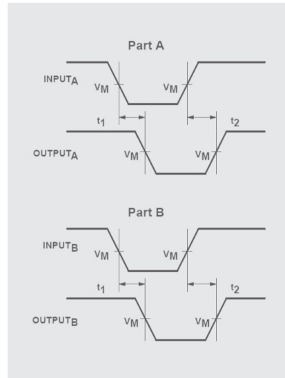
Figure 4.6 | Process Skew
