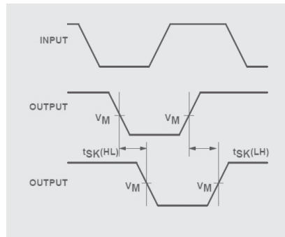
Figure 4.5 | Output skew illustration
