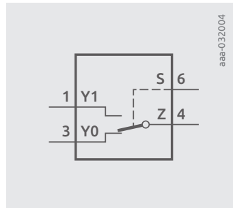
Figure 2.9 | Logic diagram SPDT switch
