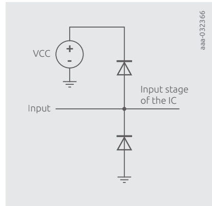
Figure 9.2 | ESD protection circuit for HC(T) input stages
