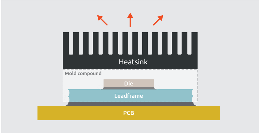
Figure 7.13 | External Heatsink on a package
