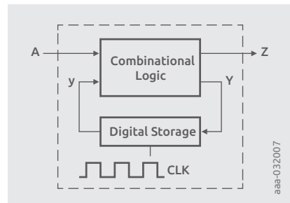
Figure 4.2 | Synchronous Logic element
