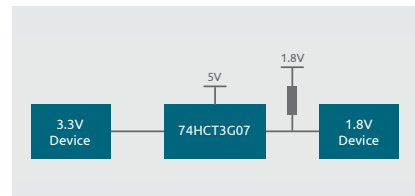
Figure 5.12 | Low threshold inputs with open drain outputs
