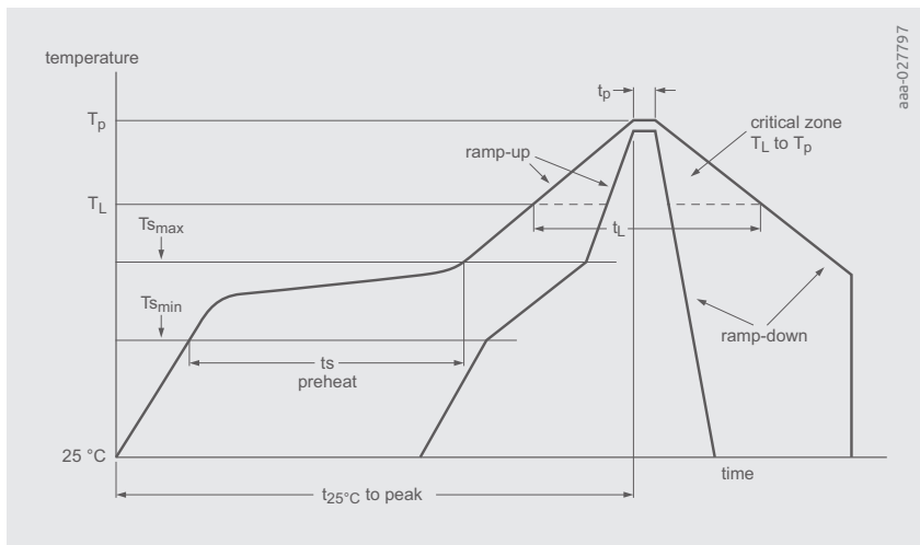
Figure 7.6 | Temperature profile of a reflow process for an XSON6 package
