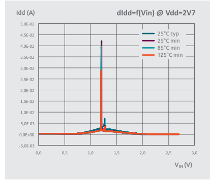
ALVT Schmitt-Trigger input curves at 2V7
