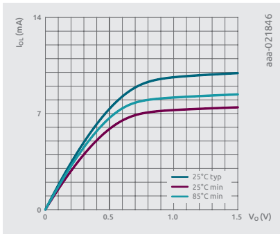
I_{OL} at 1.5V
