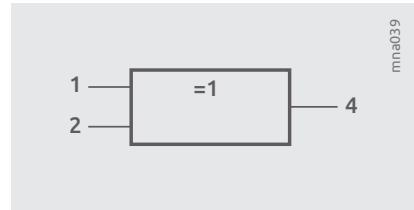
Figure 2.6b | IEC symbol of a XOR gate
