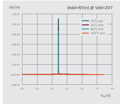
LVT Schmitt-Trigger input curves at 2V7
