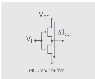
Figure 5.19 | Illustration of \Delta I_{CC} current
