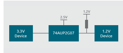
Figure 5.10 | OVT input with open drain outputs
