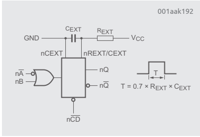
Figure 6.29 | Monostable Multivibrator
