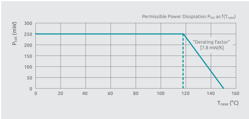
Figure 7.10 | Example of a package with a derating factor of 7.8 \text{ mW}/\text{K} starting at 118^\circ\text{C}
