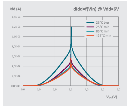
HC input curves at 6V
