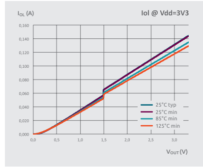
ALVT output curves at 3V3
