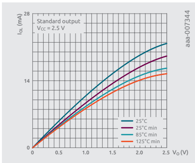
I_{OI} at 2.5V
