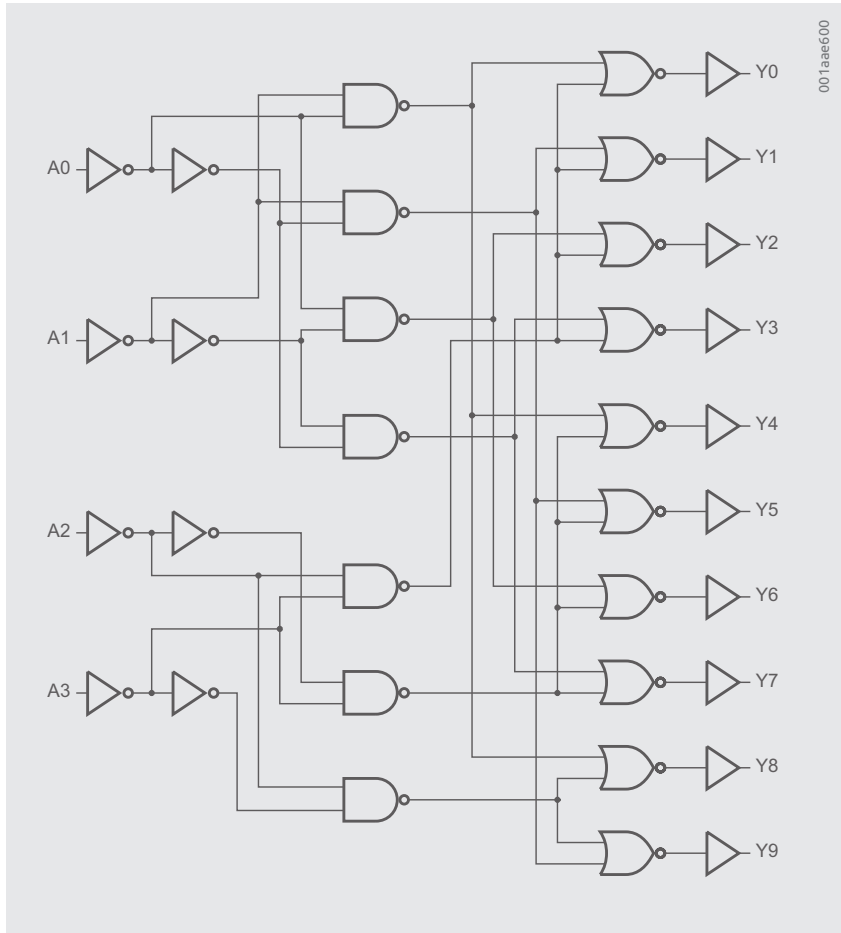
Figure 6.30 | BCD to decimal 10 outputs decoder
