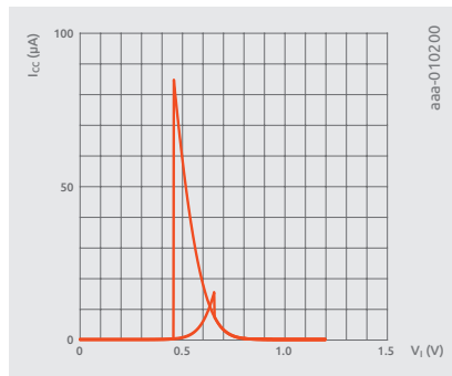
1.2V Schmitt trigger
