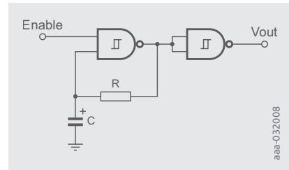
Figure 6.6 | Schmitt Trigger NAND-Gate Oscillator with output buffer gate
