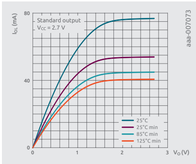
I_{OL} at 2.7 V
