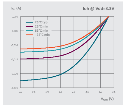
HC output curves at 3.3V
