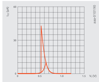
1.2V Schmitt action
