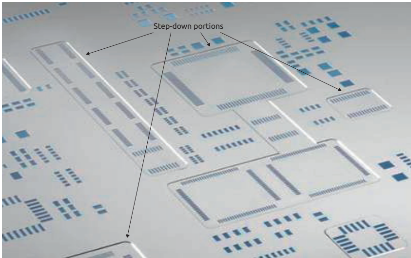
Figure 7.4 | Step down Masks on a PCB
