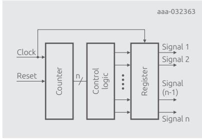
Figure 6.28 | Application example for a synchronous counter with attached decoding control network and output register
