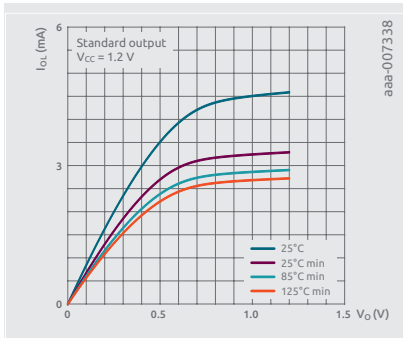
I_{OL} at 1.2 V
