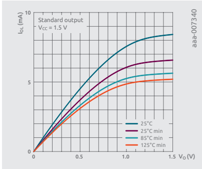
I_{OI} at 1.5V
