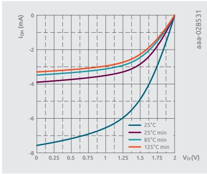
I_{OH} at 2.0V
