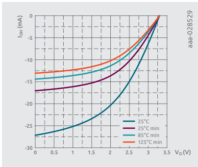
I_{OH} at 3.3V
