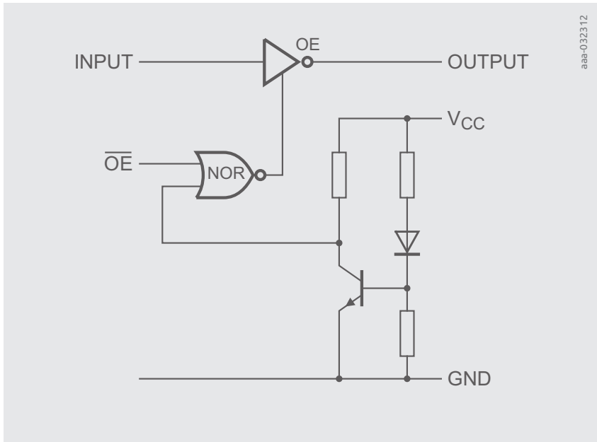
Figure 9.9 | Power-up state
