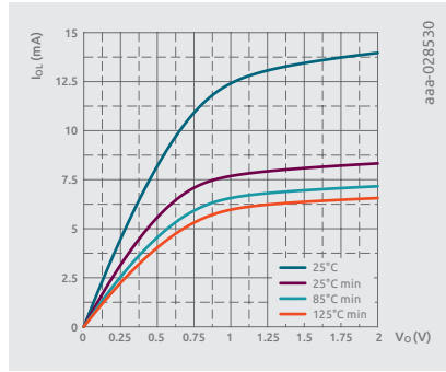
I_{OL} at 2.0V
