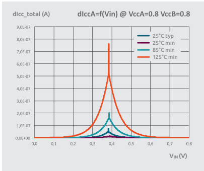
AVC input at 0.8V
