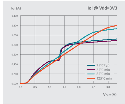
LVT output curves at 3V3
