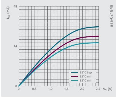
I_{OL} at 2.5V
