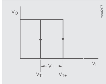
Figure 2.11 | Schmitt Trigger Input Characteristic
