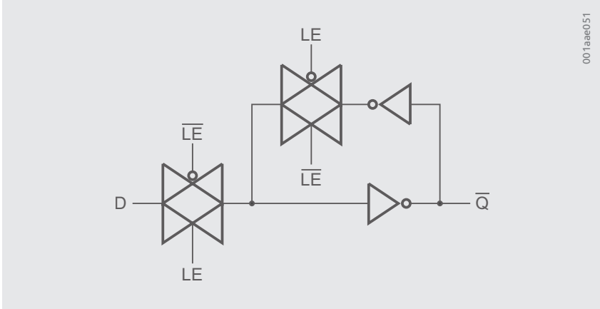
Figure 6.18 | Transparent Latch
