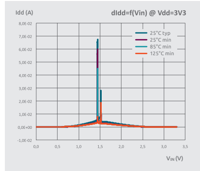
ALVT Schmitt-Trigger input curves at 3V3
