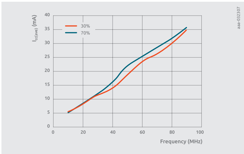
Figure 3.2 | Current consumption for different duty cycles
