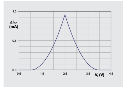
Figure 5.18 | \Delta I_{CC} current over V_I
