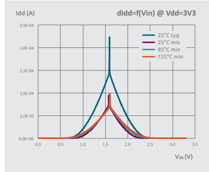
HC input curves at 3V3
