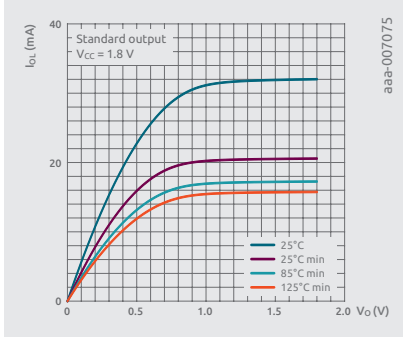
I_{OL} at 1.8 V
