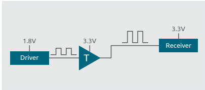
Figure 5.3 | Uni-directional low-to-high voltage translation
