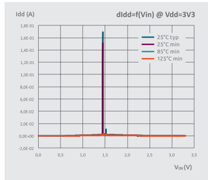
LVT Schmitt-Trigger input curves at 3V3
