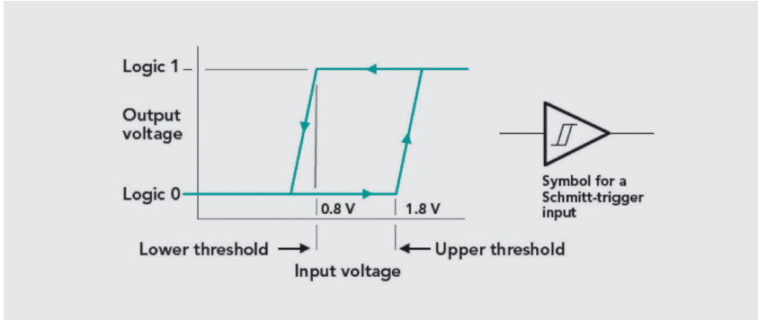
Figure 5.14 | Schmitt-Trigger Symbol and input voltage characteristics
