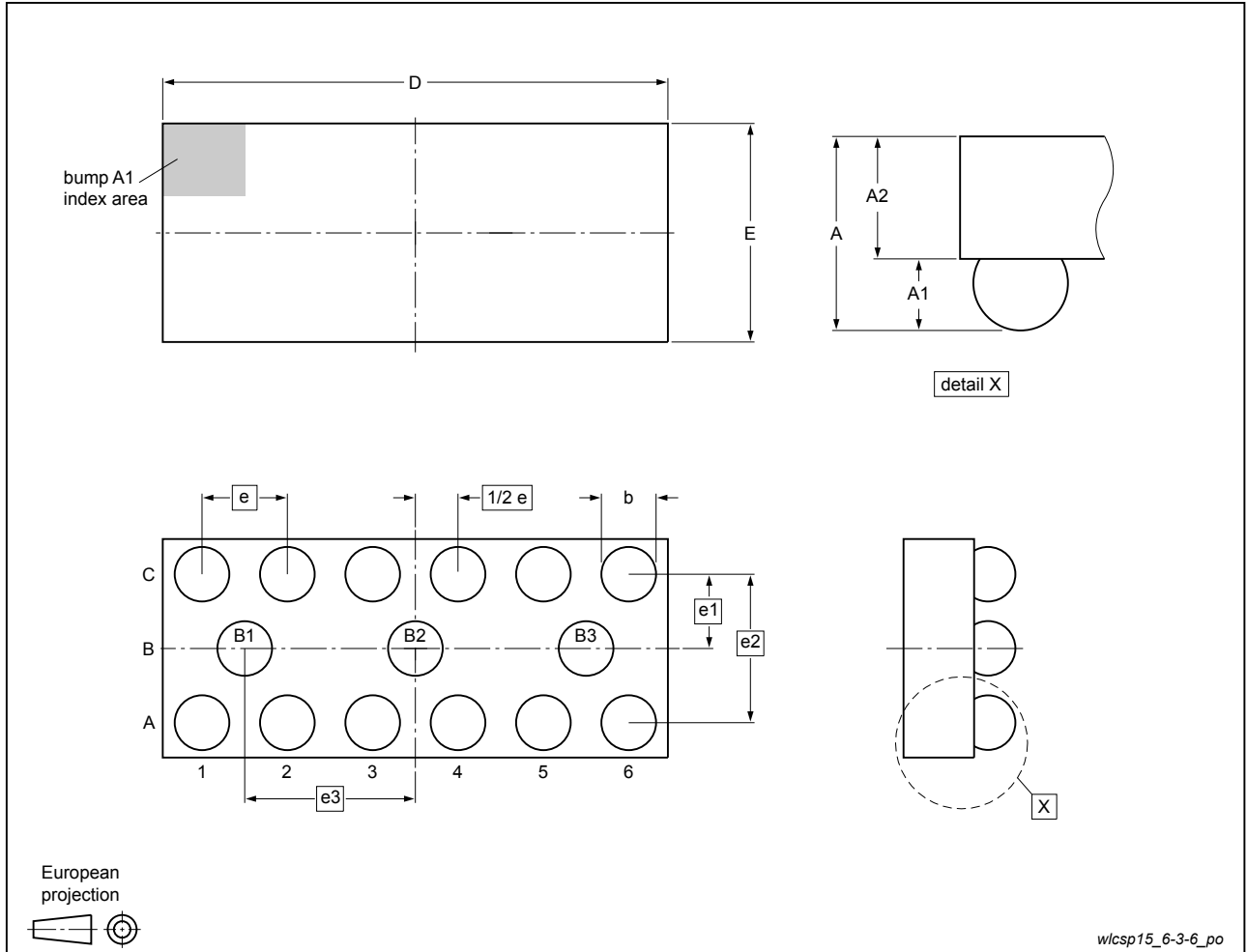
Fig. 1. Package outline WLCSP15 (WLCSP15_6-3-6)
